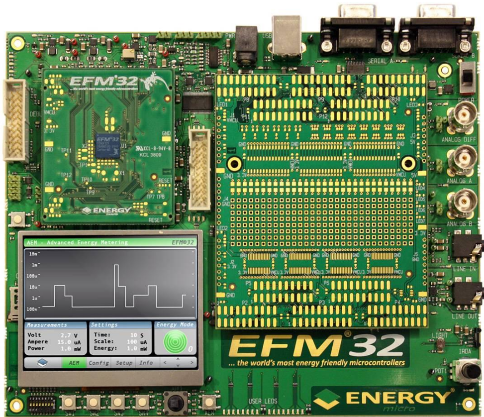
Figure 3: Development Kit
