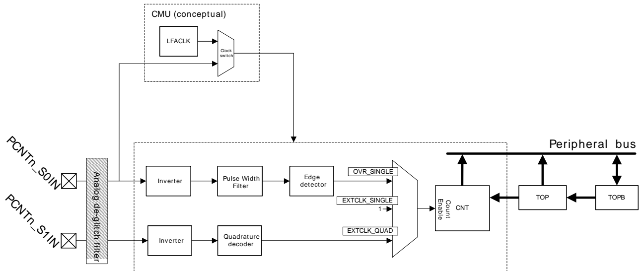
Figure 1.1. Pulse Counter Overview
