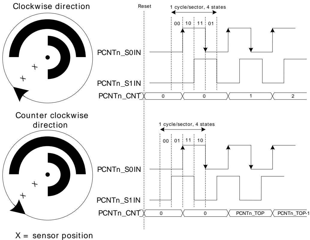
Figure 2.1. Quadrature Decoding
