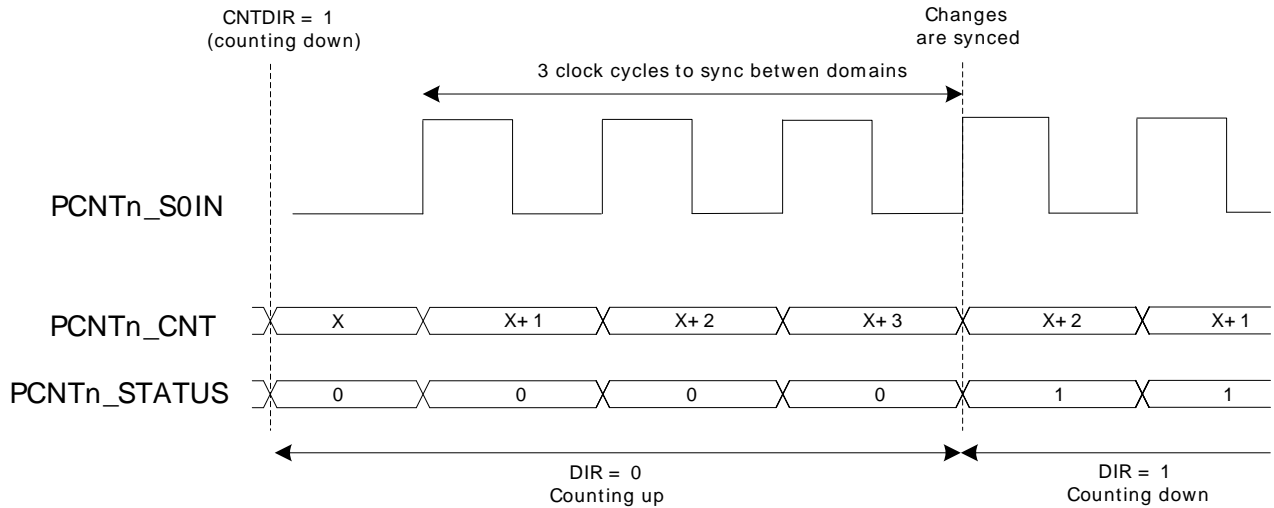
Figure 4.1. Register Sync in EXTCLKSINGLE
