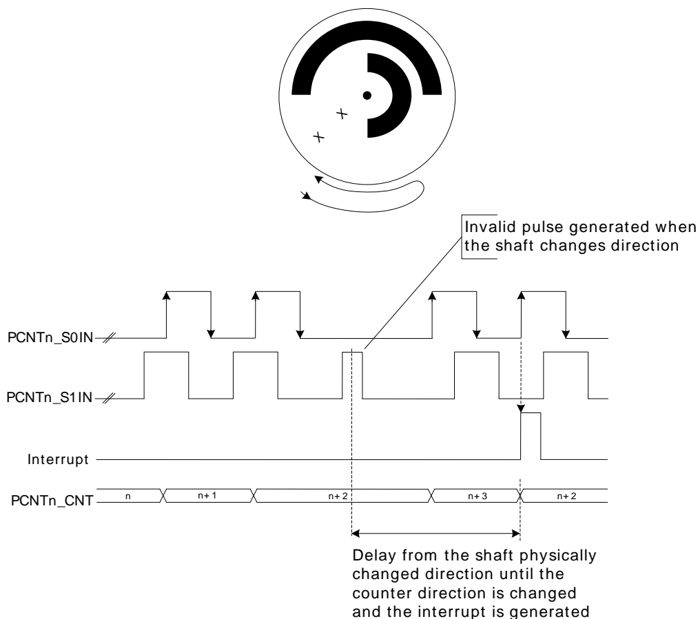
Figure 3.1. Direction Change Interrupt
