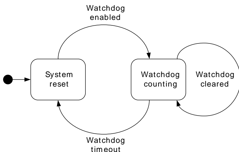
Figure 2.1. Watchdog state diagram
