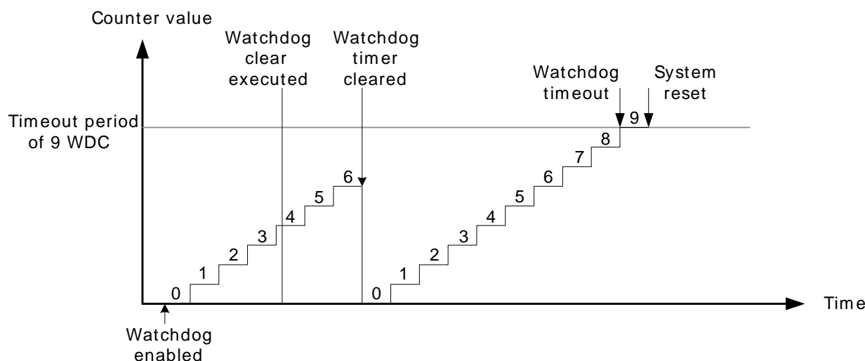
Figure 2.2. Discrete representation of the Watchdog timer operation
