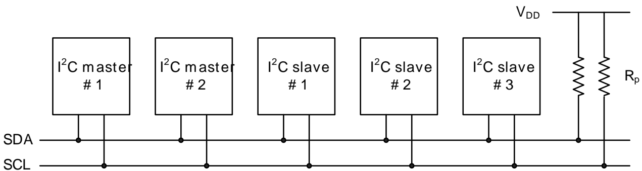
Figure 1.1. I2C Bus
