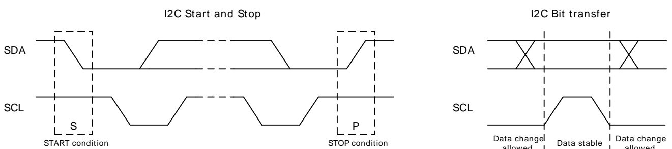
Figure 1.2. Start, Stop and Data
